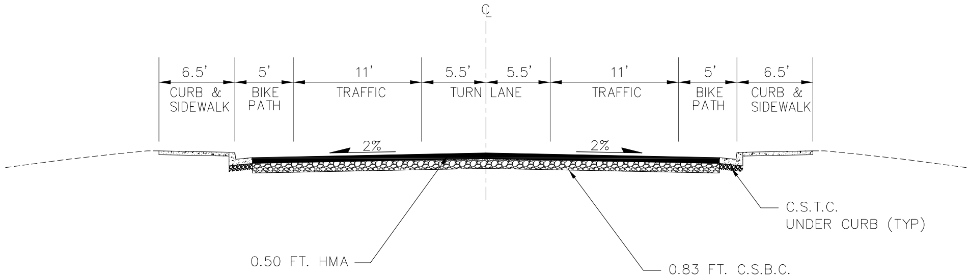
SEPARATED SIDEWALK WITH SWALE
