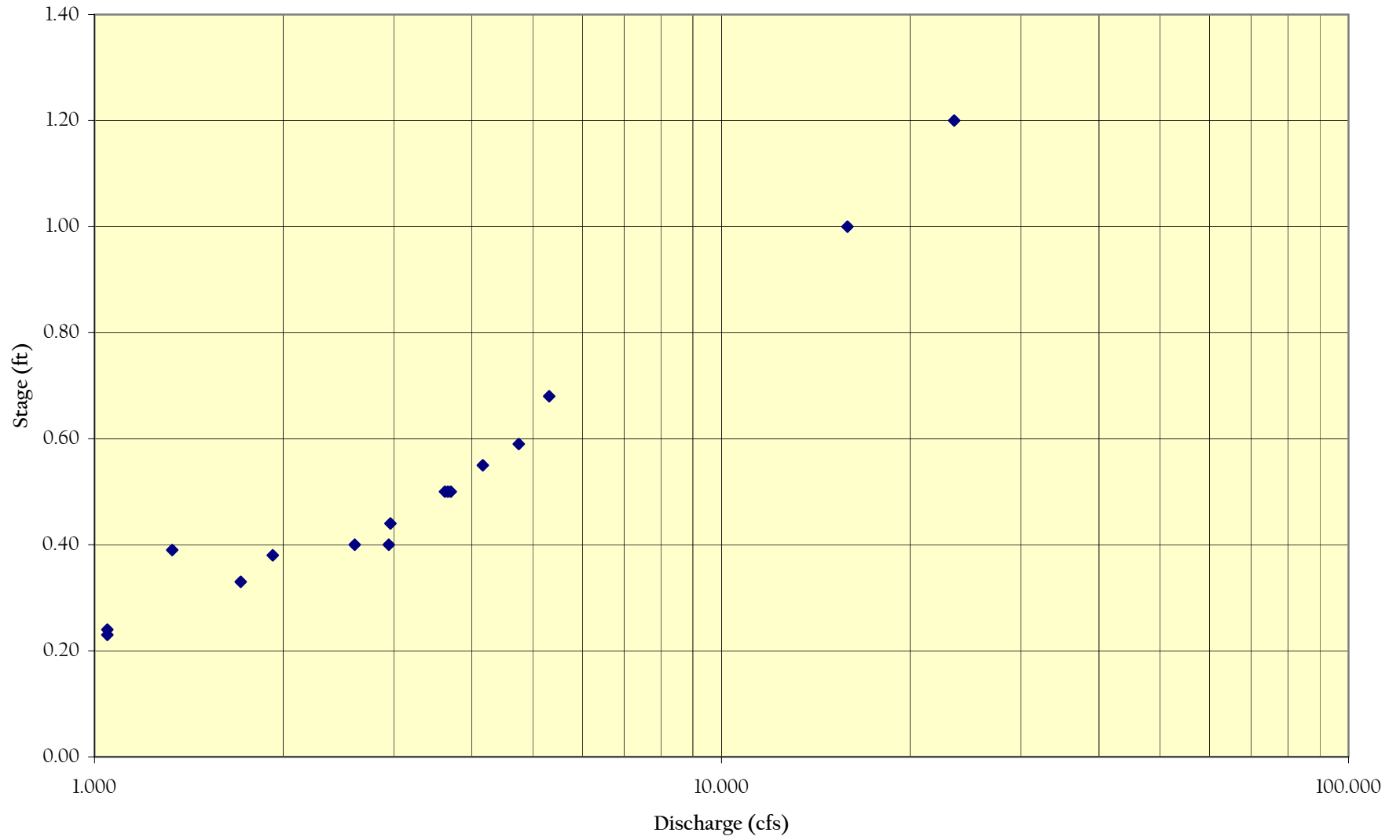
Temple Creek Rating Curve
