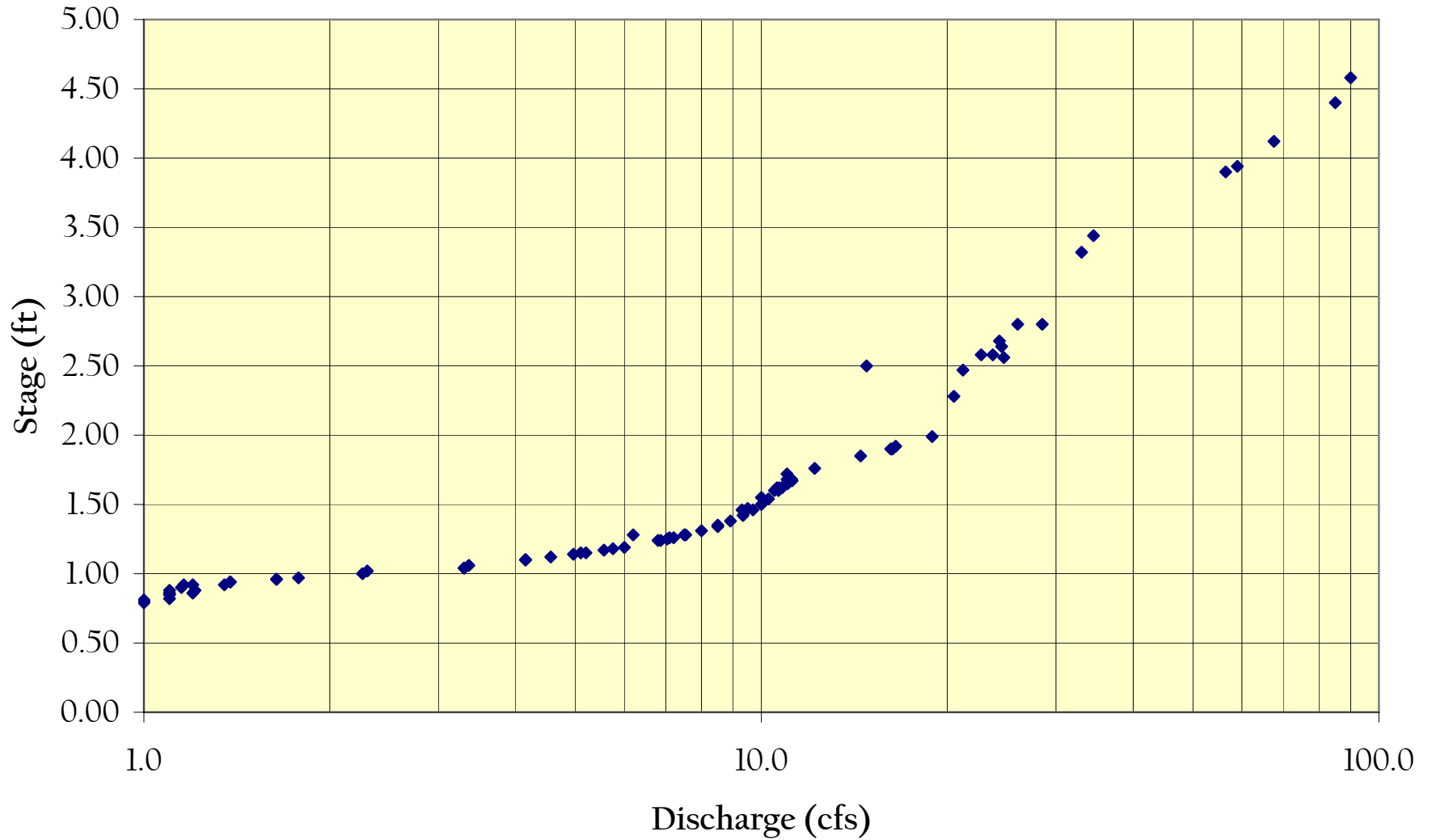
Thompson Creek Rating Curve
