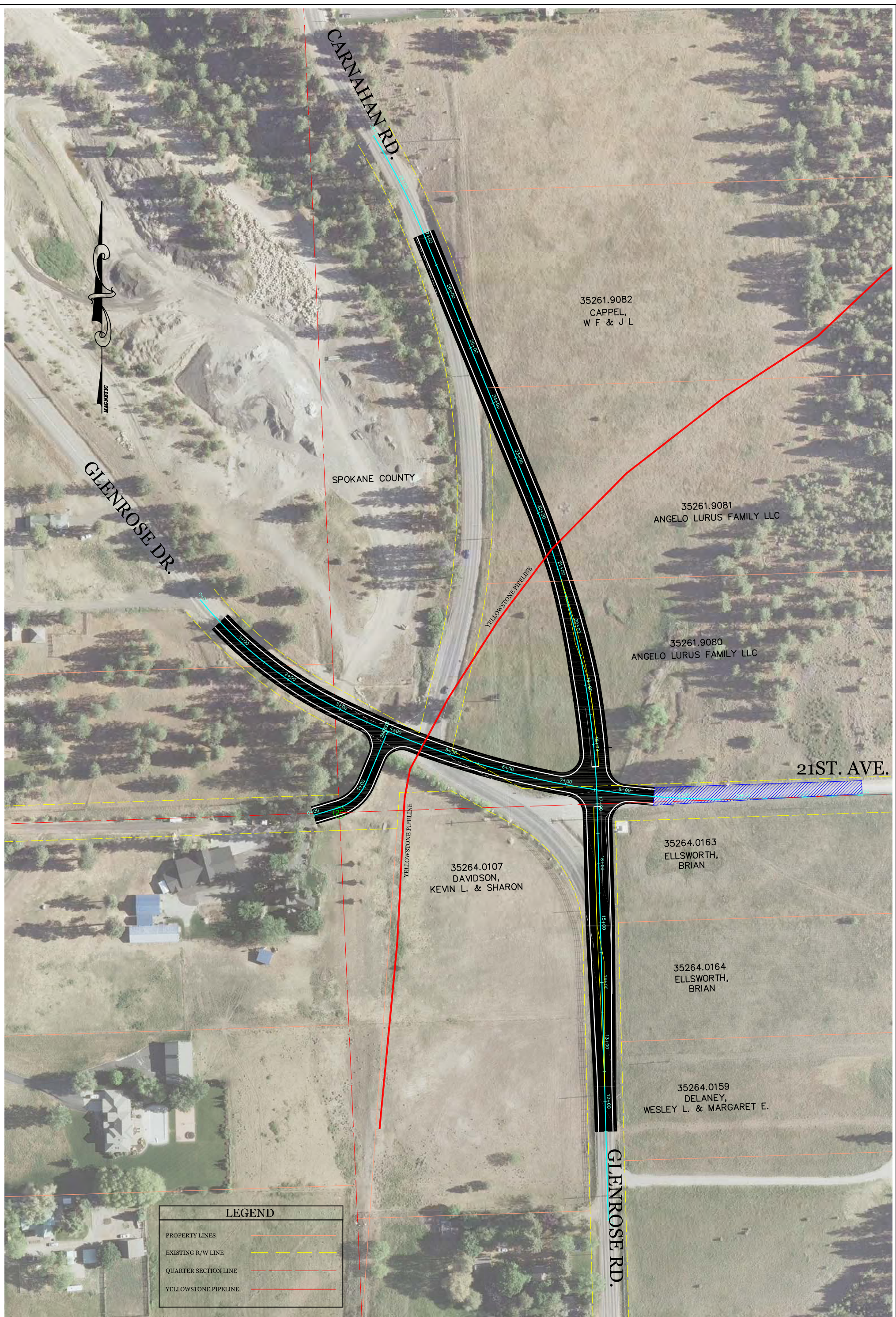
OPTION # 2 - CARNAHAN RD. / GLENROSE RD. - 4 LEG INTERSECTION
