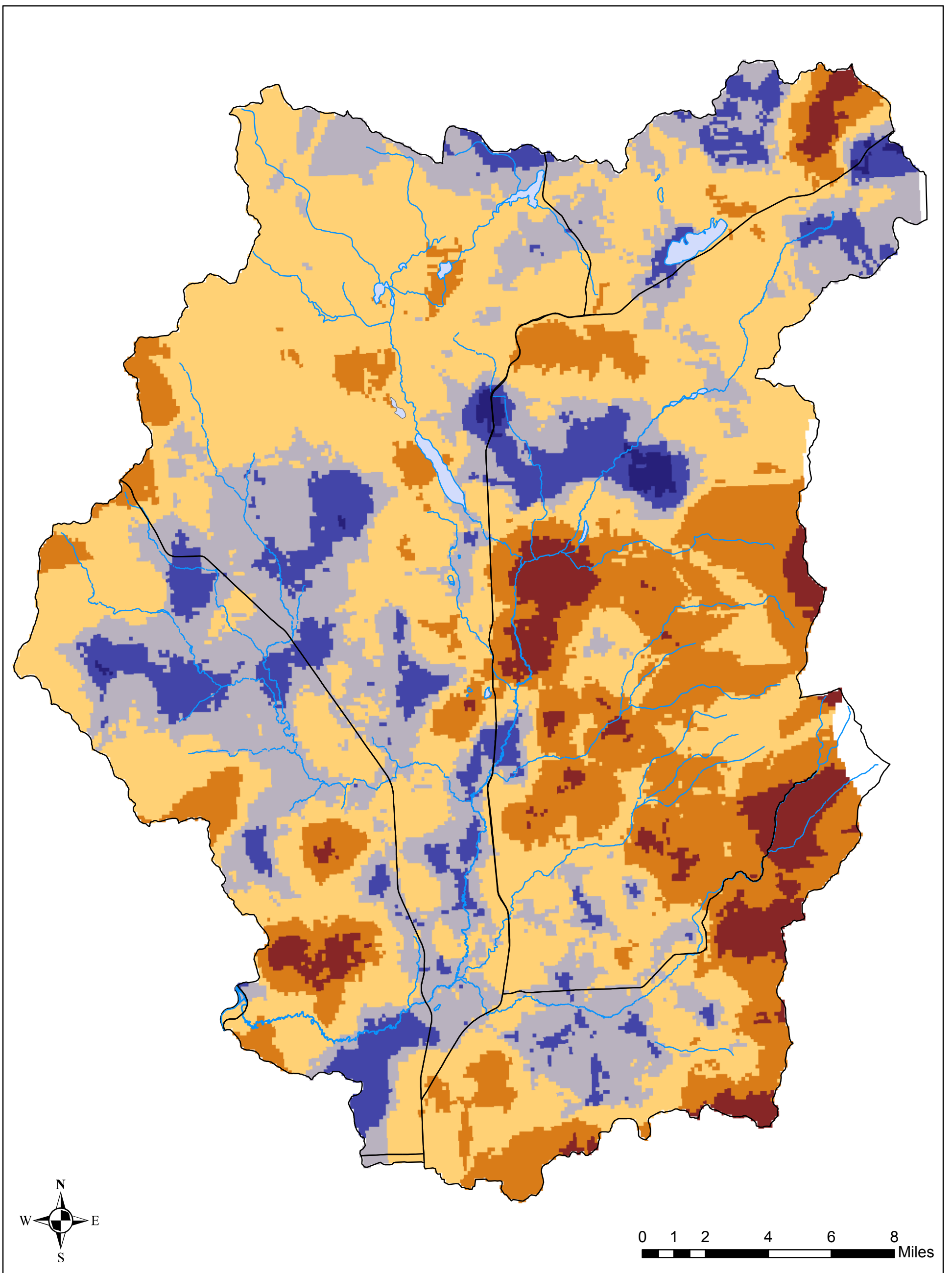
Figure 2-4 WRIA 55 Water Well Total Depth Spatial Variation
