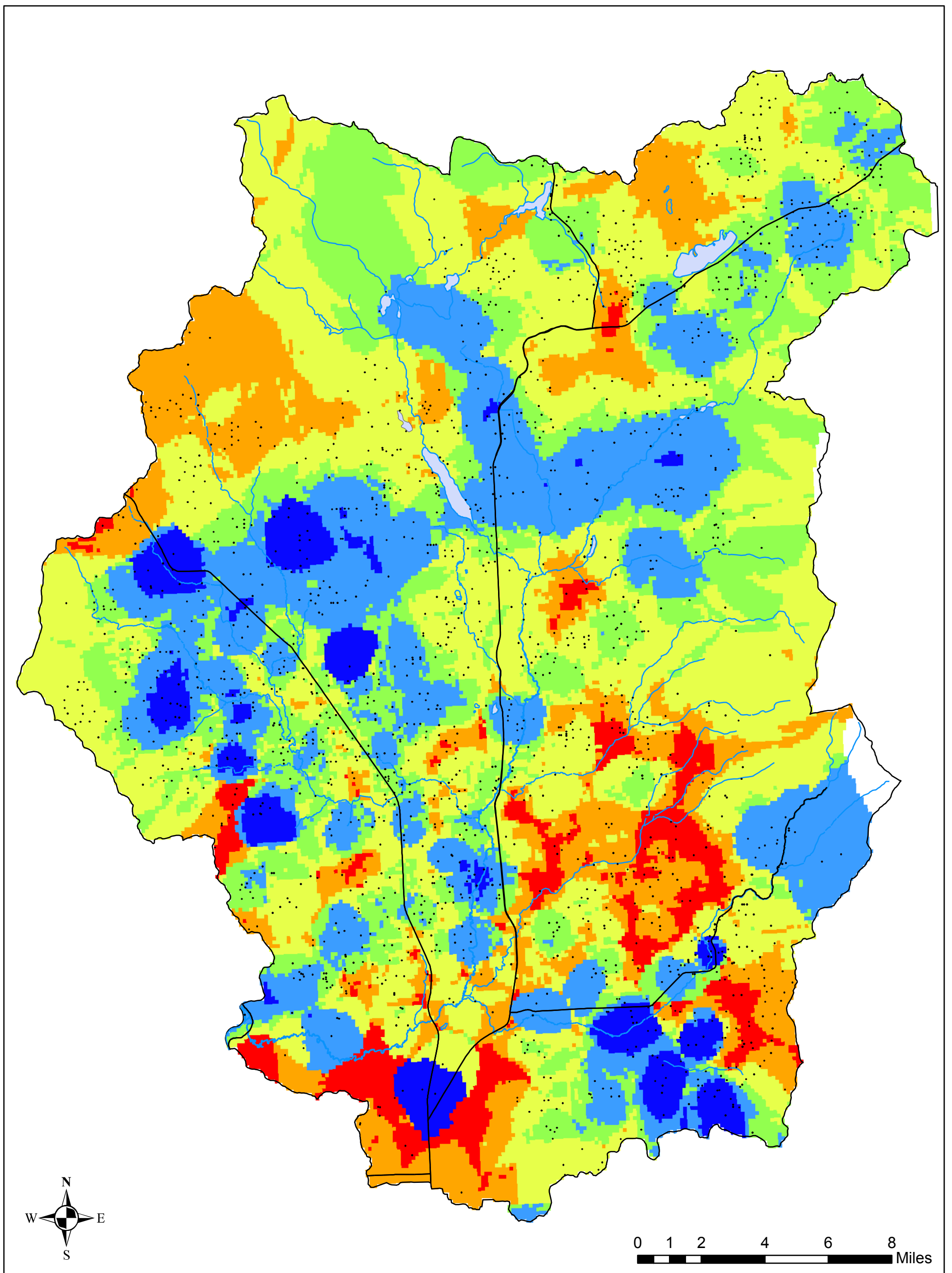
Figure 2-3 WRIA 55 Water Well Yield Spatial Variation
