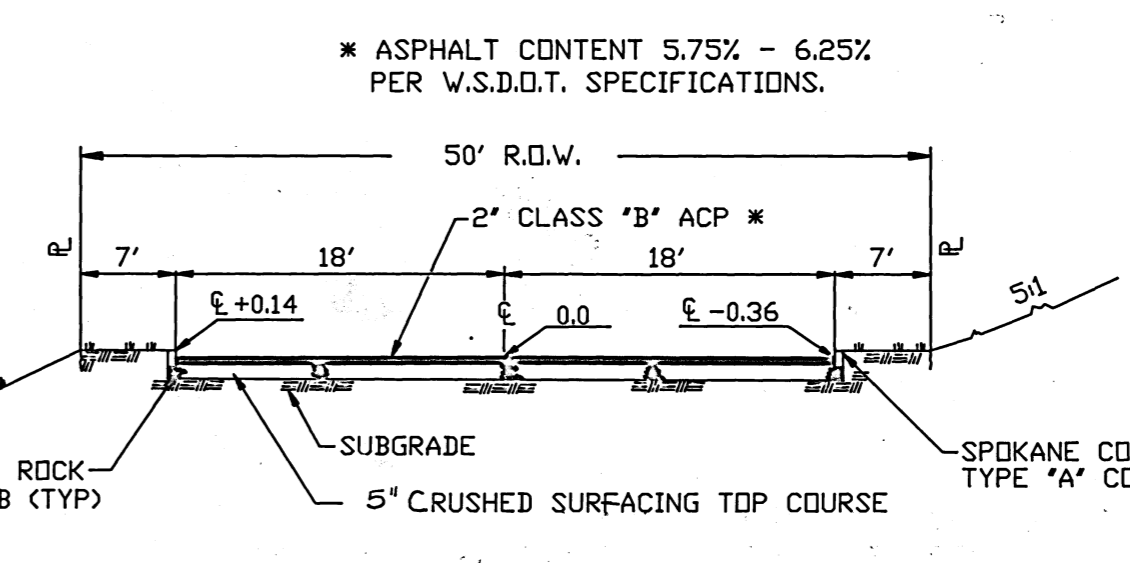
1 TYPICAL CROWNED STREET SECTION NTS
