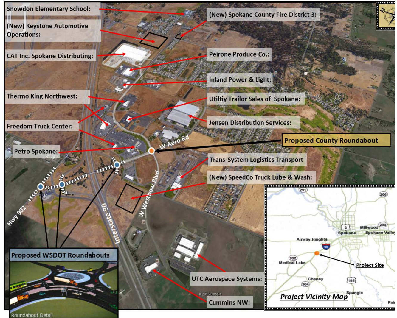
Proposed Roundabout at West Westbow Boulevard and West Aero Road
