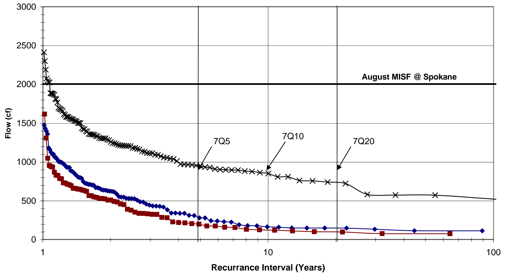
FIGURE 5.6b: Recurrence Interval of 7-Day Average Minimum Flows in WRIA 67
