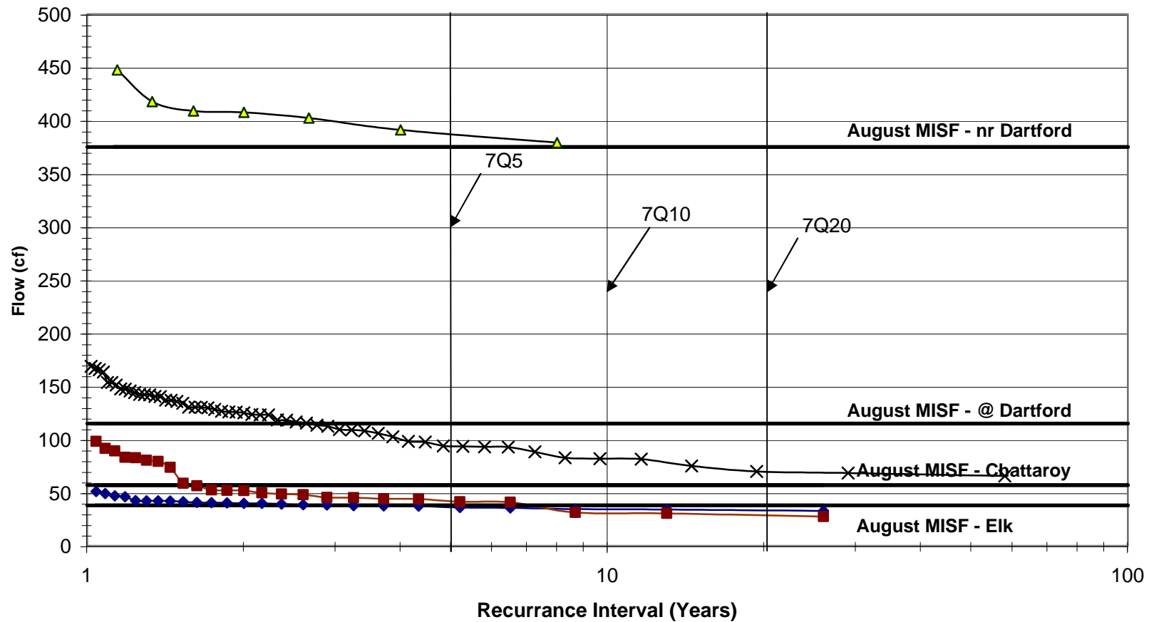
FIGURE 5.6a: Recurrence Interval of 7-Day Average Minimum Flows in WRIA 55
