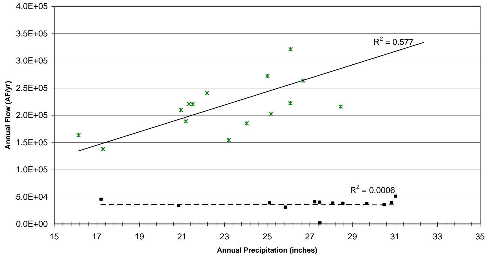
FIGURE 5.4a: Total Annual Flow Volume vs Total Annual Precipitation - WRIA 55
