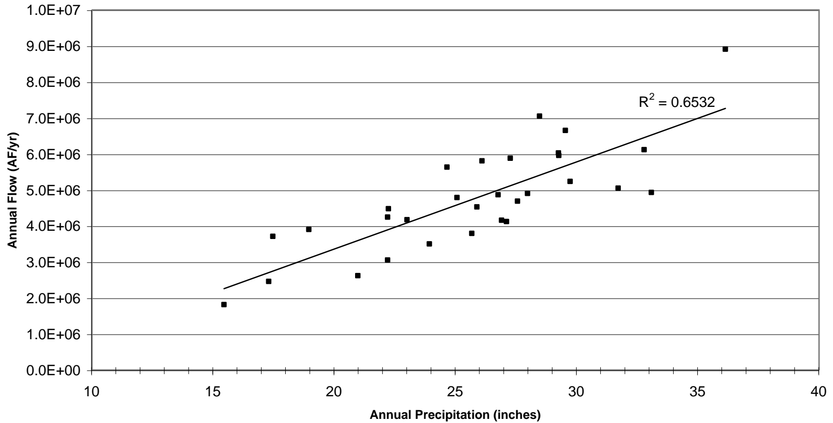
FIGURE 5.4b: Total Annual Flow Volume vs Total Annual Precipitation - WRIA 57
