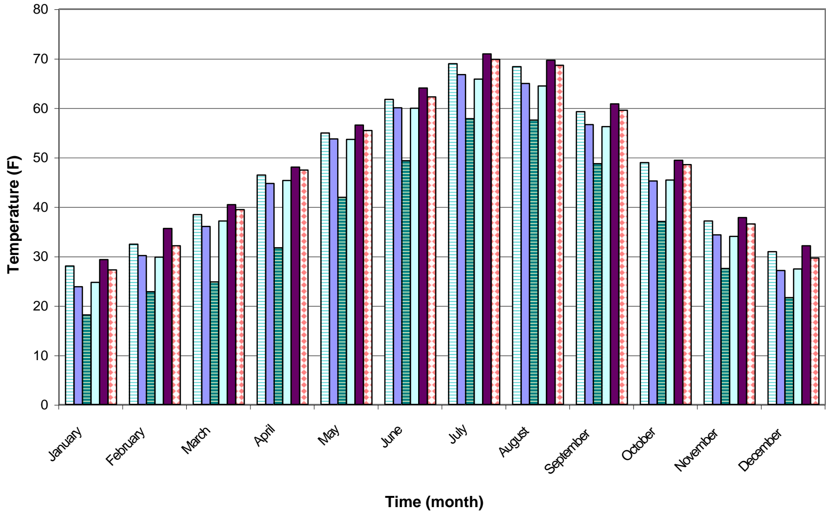
FIGURE 4.9: Mean Monthly Temperature Spokane County Watershed Assessment
