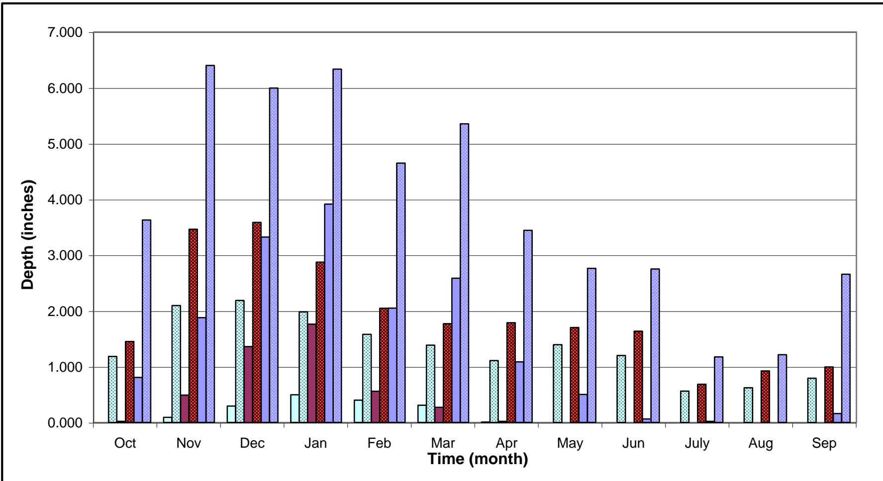
FIGURE 4.8: Monthly Precipitation (PRCP) vs. Snow Water Equivalent (SWE)
