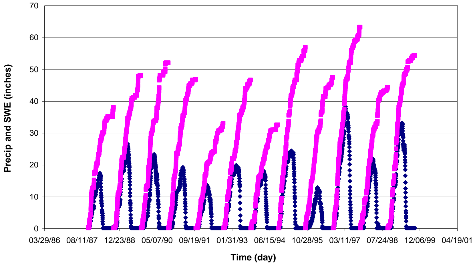
FIGURE 4.7a: Accumulated Daily Precipitation and Snow Water Equivalent (SWE) - Quartz Peak, stn 45031
